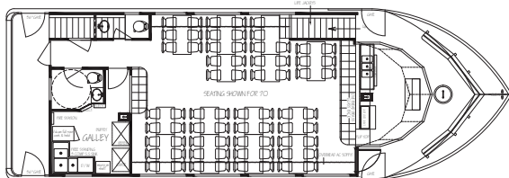
MAIN DECK ARRANGEMENT
